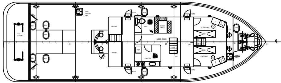
MAIN DECK
