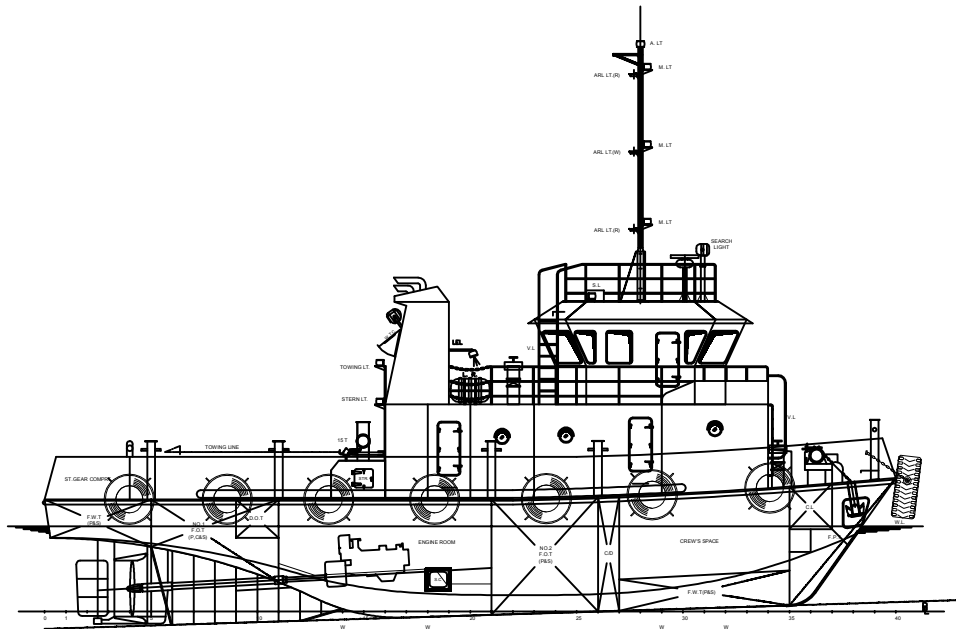
PROFILE DECK
